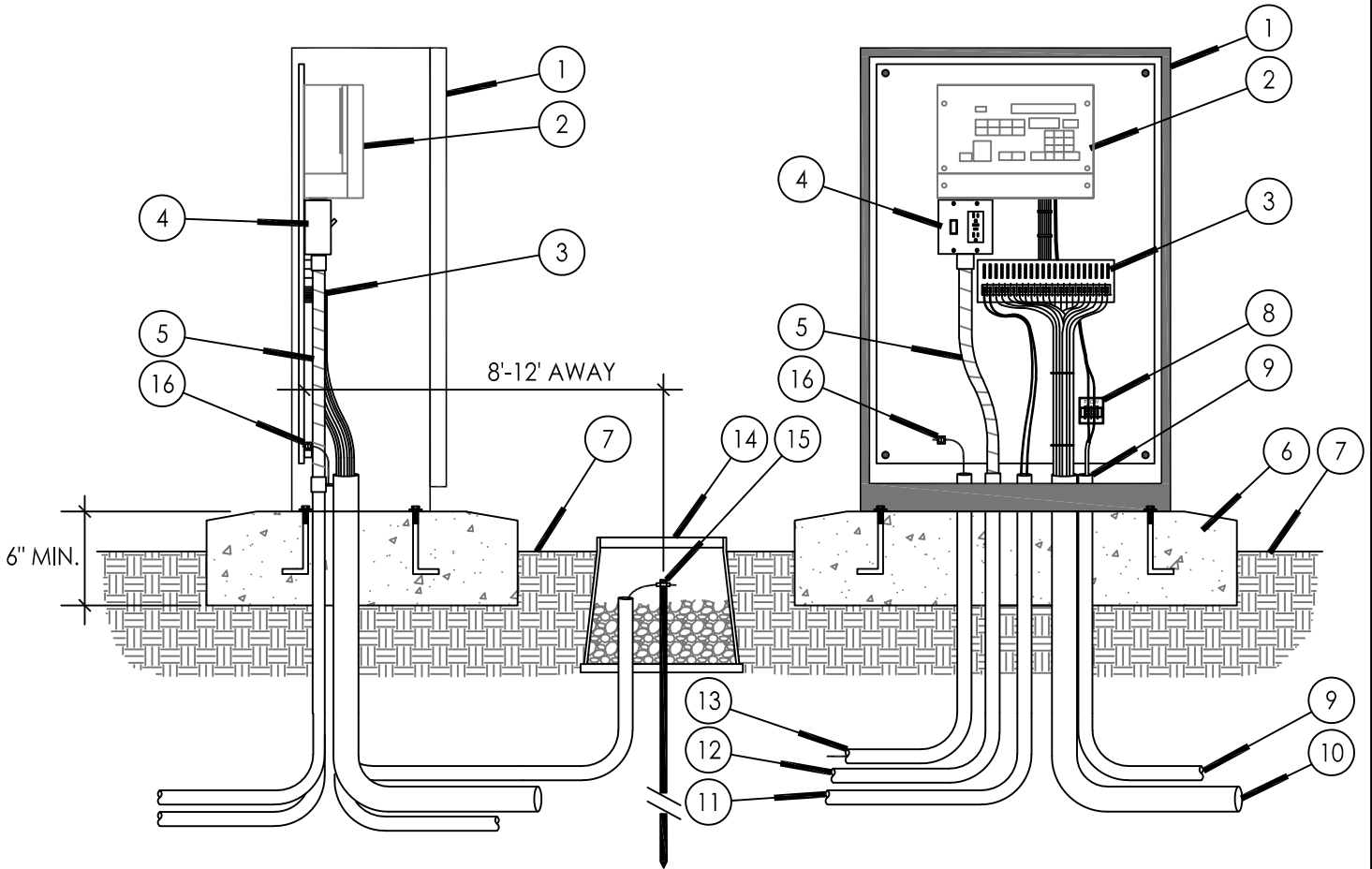
SIDE VIEW
