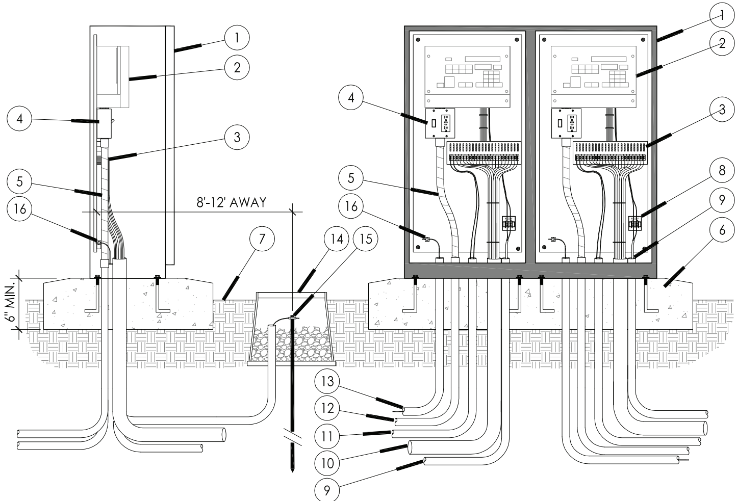
SIDE VIEW
